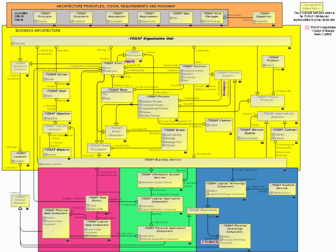
Full Metamodel Diagram for TOGAF 9
