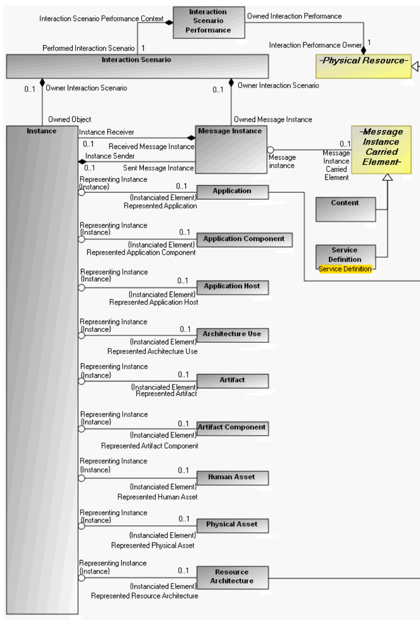
SV-10c Metamodel
