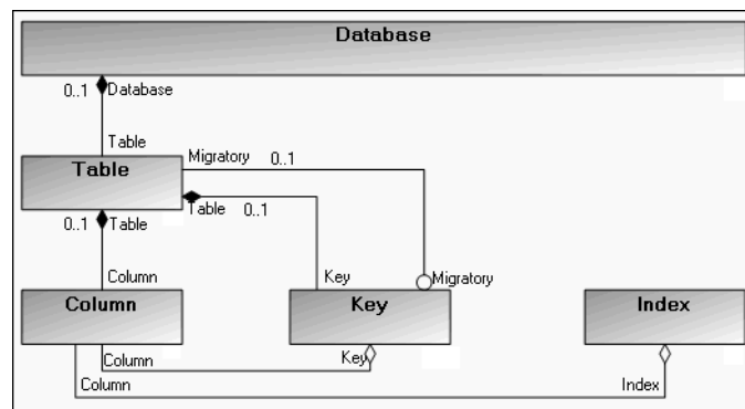
DIV-3 Metamodel
