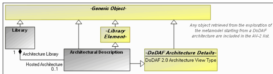
AV-2 Metamodel
