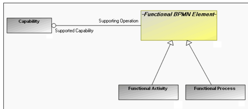
CV-6 Metamodel
