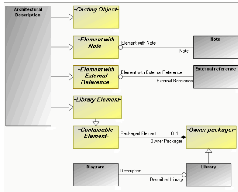
OV-1 Metamodel
