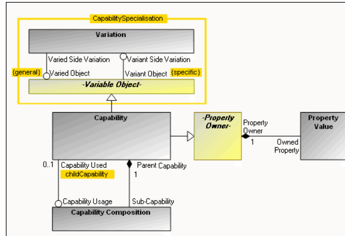
CV-2 Metamodel
